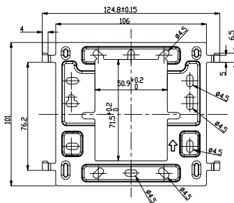
Wall bracket (DIM:mm)
